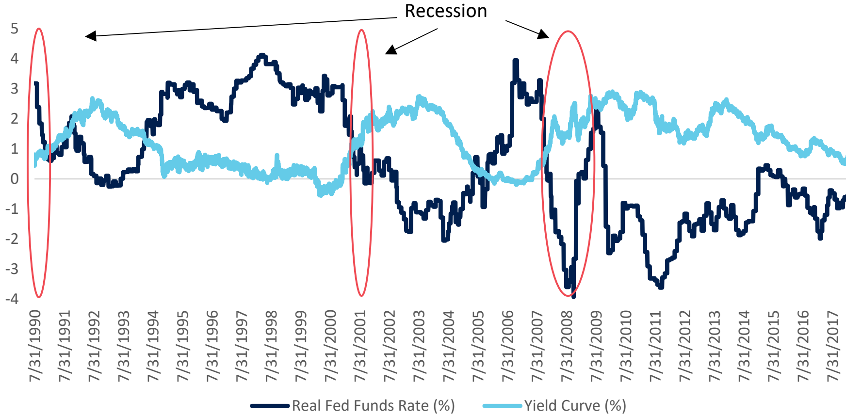
Real Fed Funds Rate (Nominal Fed Funds - Inflation) vs. Yield Curve
